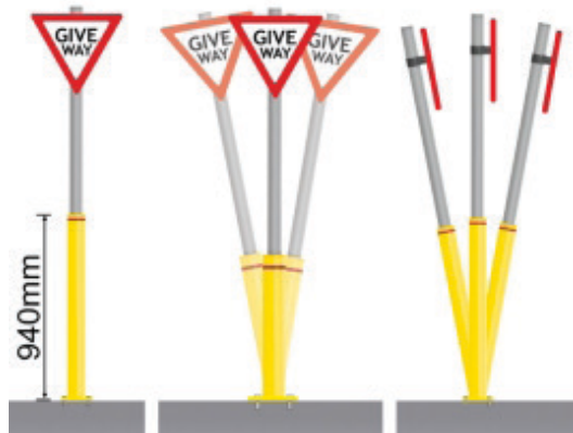
DB90/FPB - Bolt down DB90/FPI - In-ground
